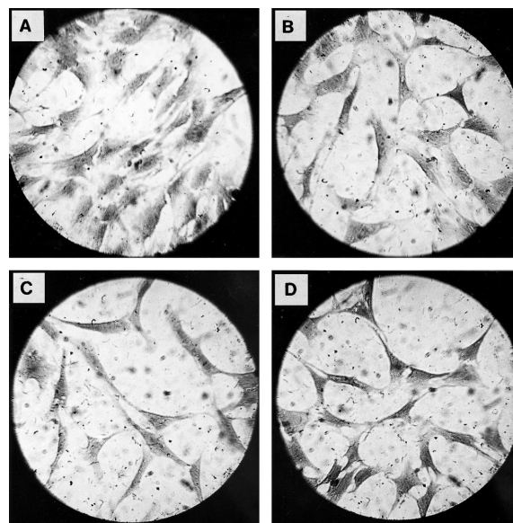
Figure 5. Effect of vanadium compounds on Swiss 3T3 fibroblast morphology. Cells were incubated in DMEM (control, A), or \mu M of vanadyl (B), vanadate (C) or pervanadate (D) for 24 h. After this period, cells were stained with crystal violet. Objective \times 40 .
